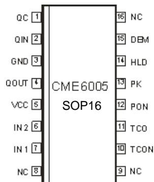
Figure 3 Pin Layout SOP16
